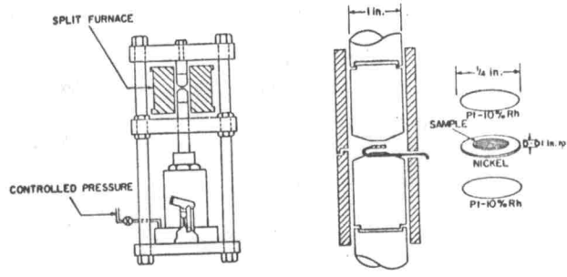
Fig. 1. Sketch of opposed anvil apparatus with enlarged views of anvil and sample assemblies
